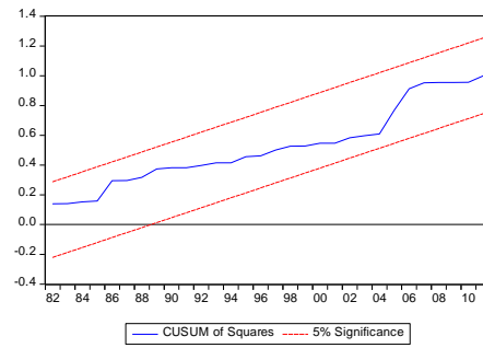
Fig. 1b: Plot of CUSUMSQ
