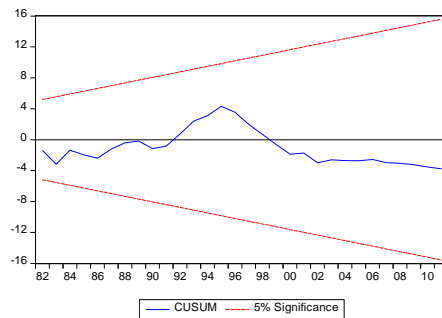
Fig. 2a: Plot of CUSUM test
