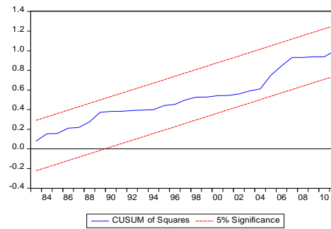
Fig. 3b: Plot of CUSUMSQ
