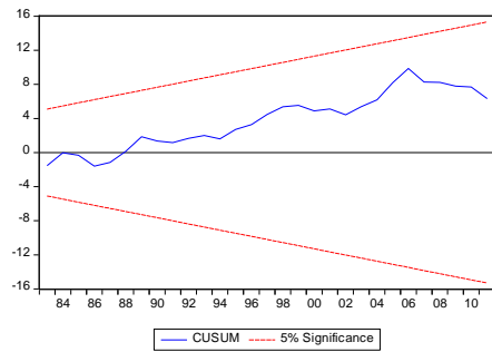
Fig. 3a: Plot of CUSUM test
