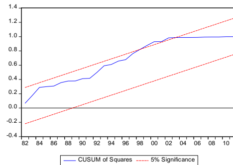
Fig. 2b: Plot of CUSUMSQ
