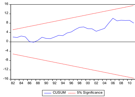
Fig. 1a: Plot of CUSUM test
